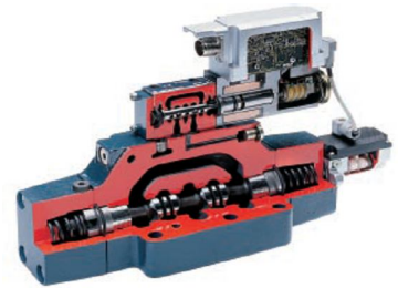
Bosch valve cutaway
