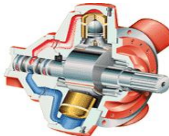
Radial motor cutaway
